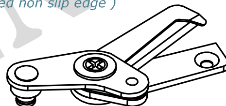
CUTTER ASSEMBLY TYPE C ▶ 5330C-0C
