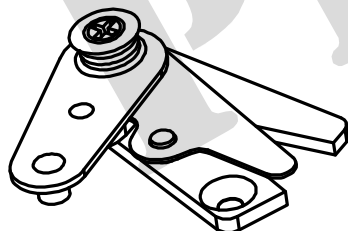
SCISSOR ASSEMBLY ▶ 5340C-00 008-68190-61XC
