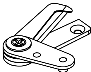
CUTTER ASSEMBLY TYPE A ▶ 5330C-0A
