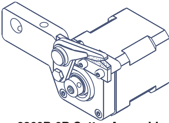
2360B-0R Cutter Assembly 2360B-00R Cutter Assembly With Stepper Motor RH ( Brazedtip Cutter )
